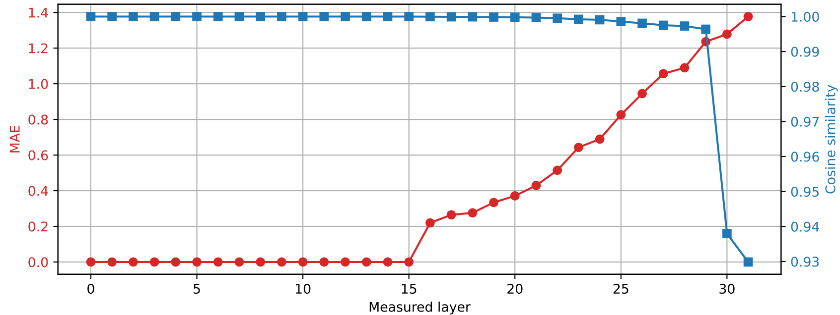
Phi-3-mini-4k-instruct | Prompt 4 Spared layer 15 | Hybrid vs quantized
