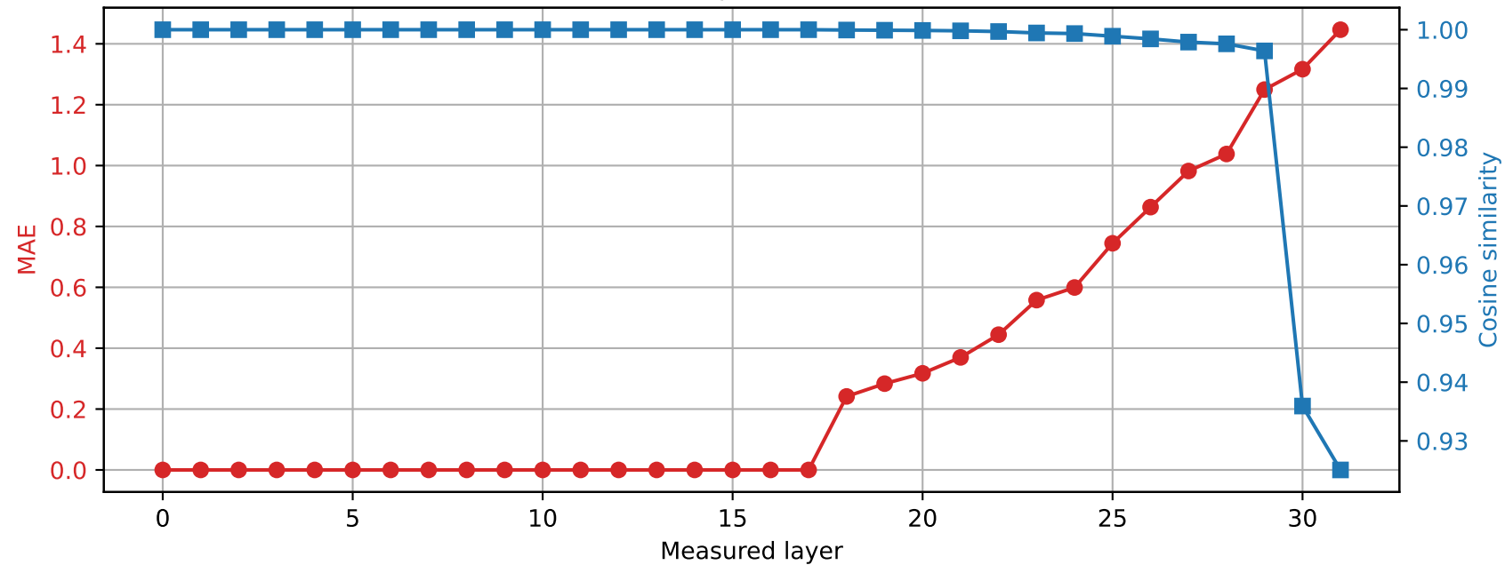
Phi-3-mini-4k-instruct | Prompt 4 Spared layer 17 | Hybrid vs quantized
