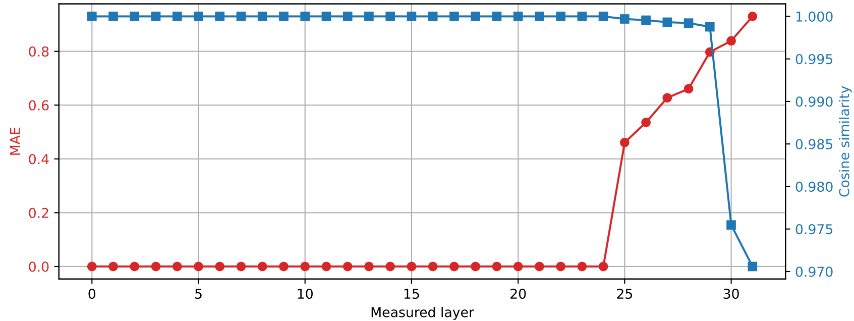
Phi-3-mini-4k-instruct | Prompt 4 Spared layer 24 | Hybrid vs quantized
