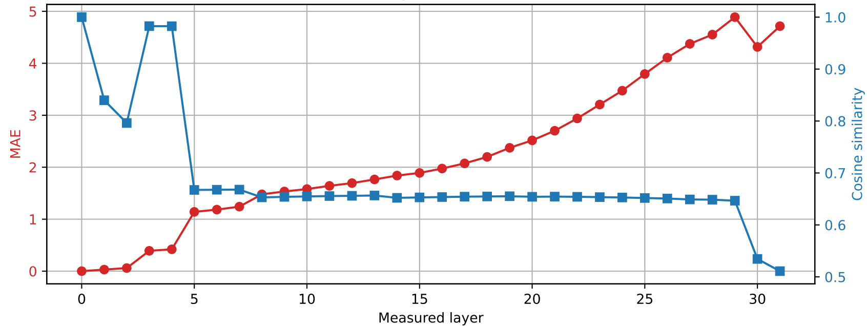
Phi-3-mini-4k-instruct | Prompt 4 Spared layer 25 | Hybrid vs unquantized
