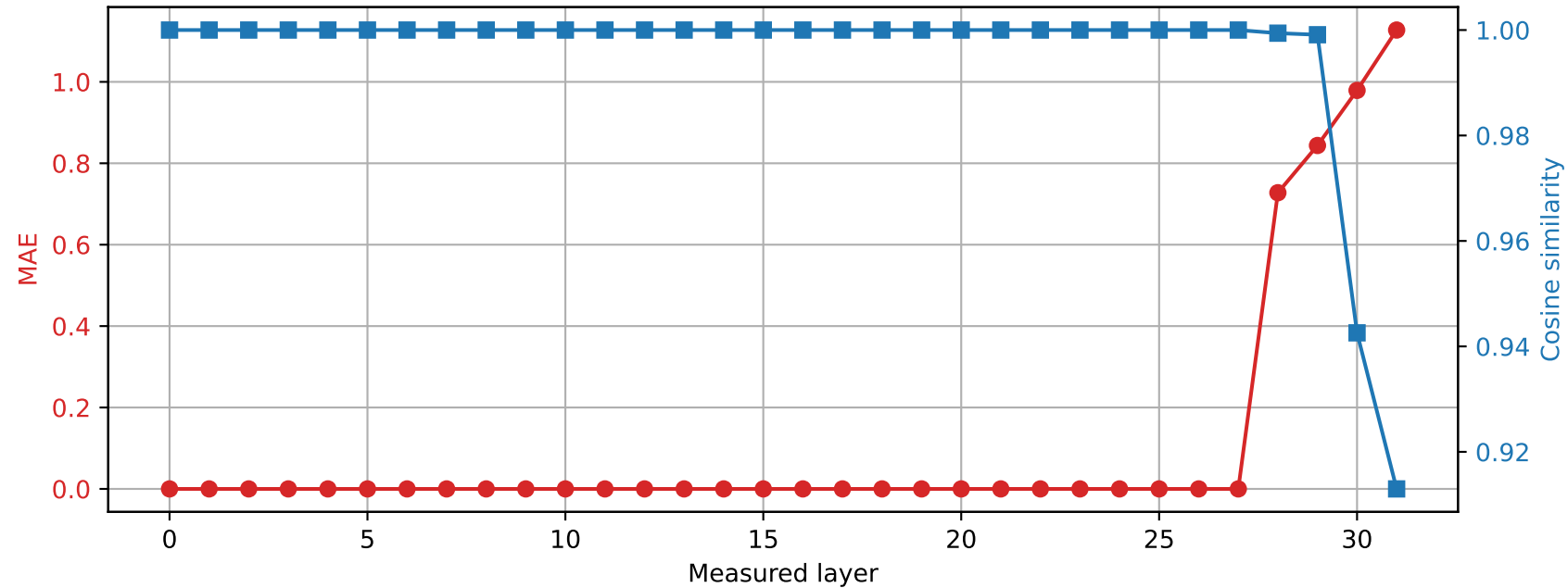
Phi-3-mini-4k-instruct | Prompt 4 Spared layer 27 | Hybrid vs quantized
