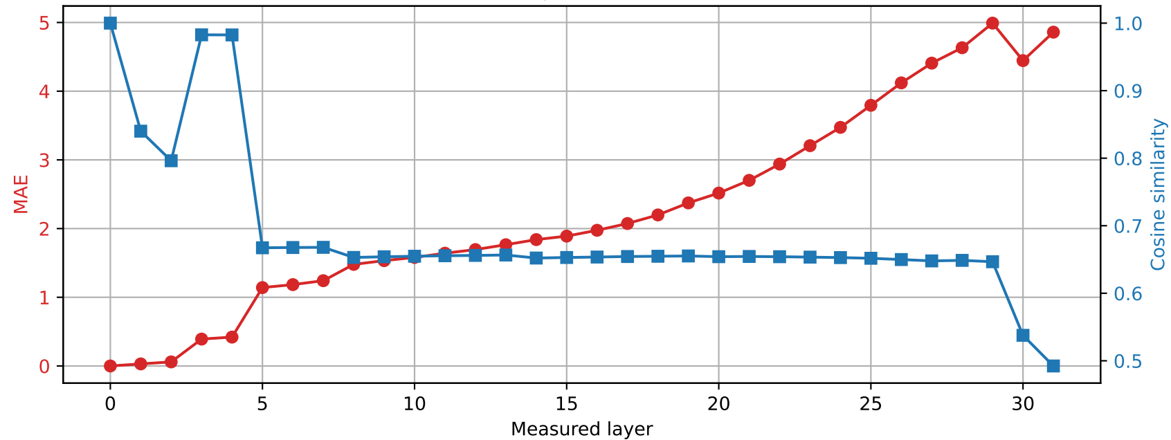
Phi-3-mini-4k-instruct | Prompt 4 Spared layer 27 | Hybrid vs unquantized
