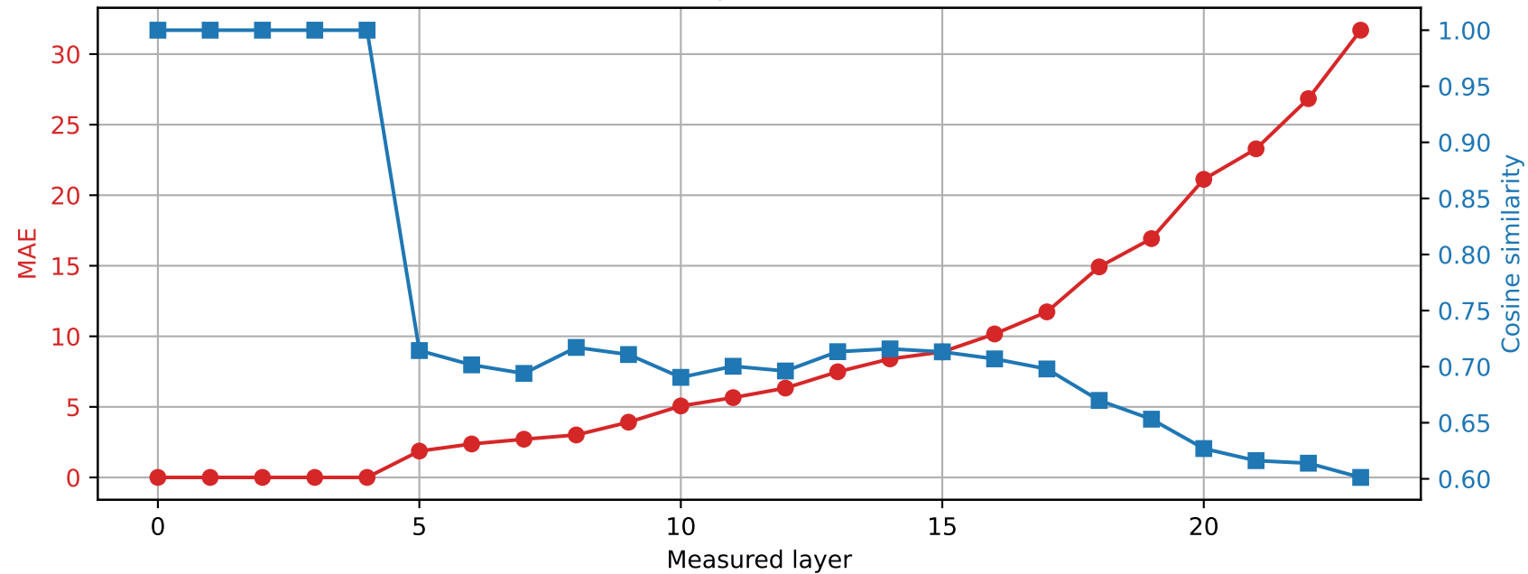
SmolLM2-1.7B-Instruct | Prompt 0 Spared layer 4 | Hybrid vs quantized
