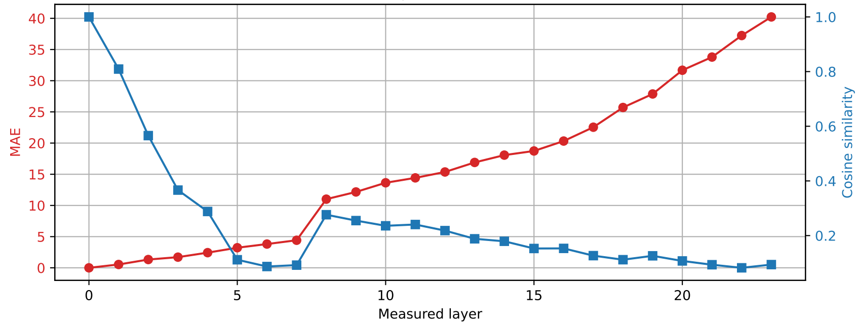
SmolLM2-1.7B-Instruct | Prompt 0 Spared layer 10 | Hybrid vs unquantized
