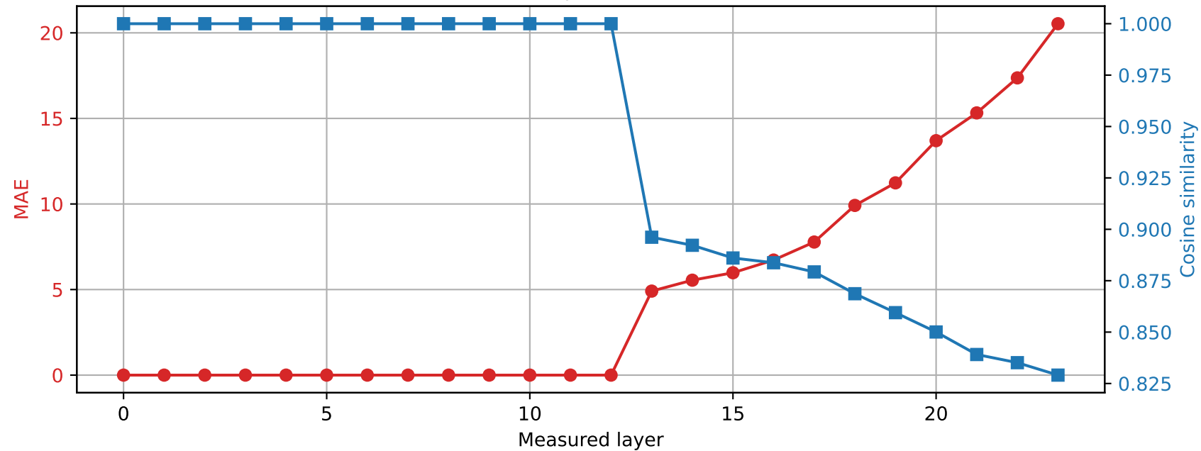
SmolLM2-1.7B-Instruct | Prompt 0 Spared layer 12 | Hybrid vs quantized
