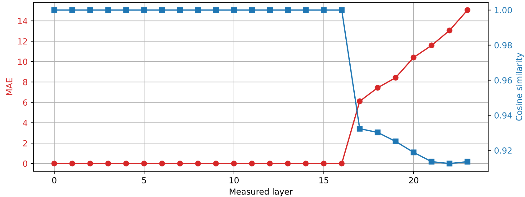
SmolLM2-1.7B-Instruct | Prompt 0 Spared layer 16 | Hybrid vs quantized
