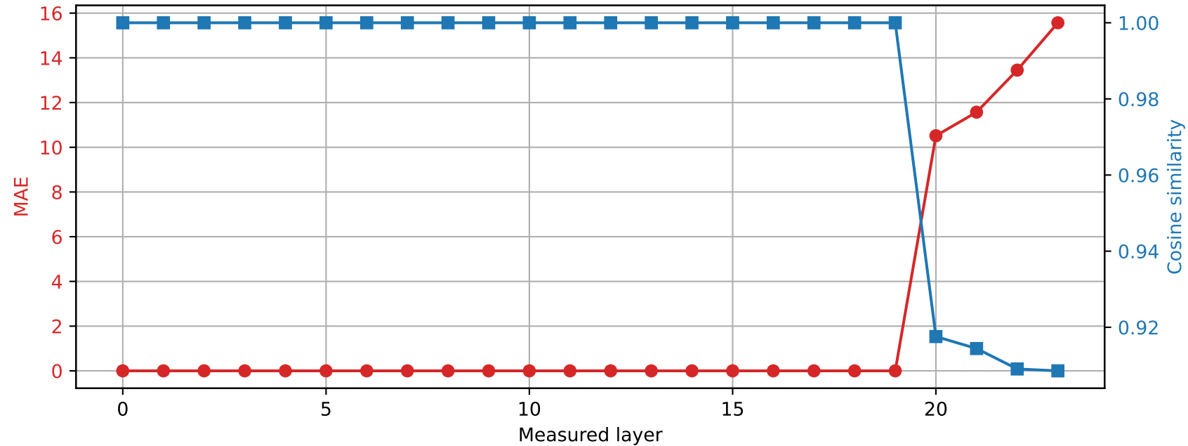
SmolLM2-1.7B-Instruct | Prompt 0 Spared layer 19 | Hybrid vs quantized
