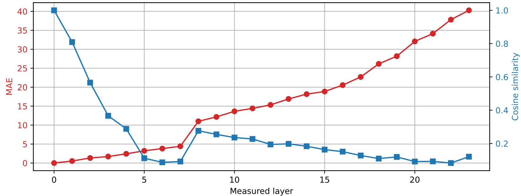
SmolLM2-1.7B-Instruct | Prompt 0 Spared layer 19 | Hybrid vs unquantized
