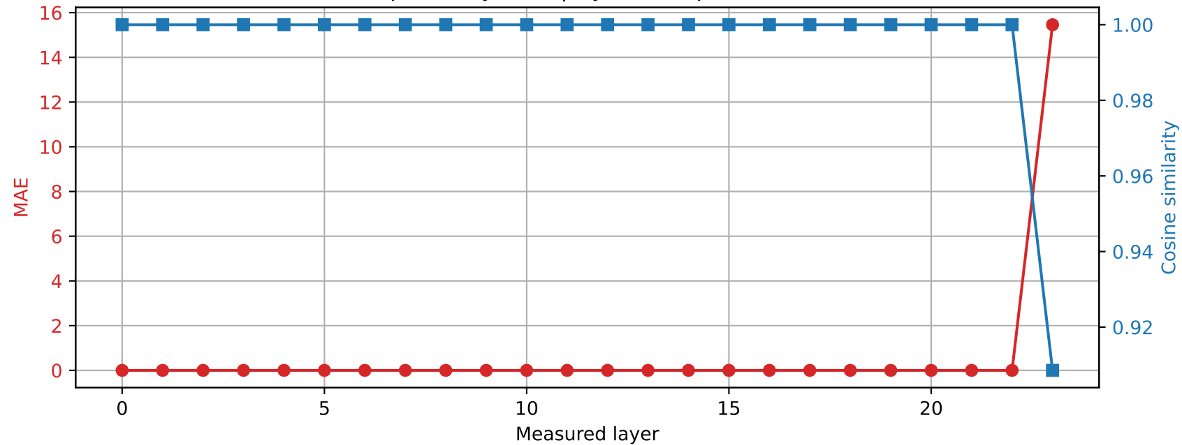
SmolLM2-1.7B-Instruct | Prompt 0 Spared layer 22 | Hybrid vs quantized
