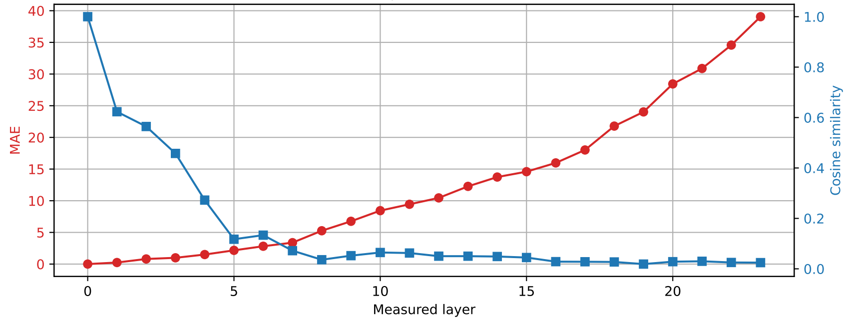
SmolLM2-1.7B-Instruct | Prompt 1 Spared layer 1 | Hybrid vs unquantized
