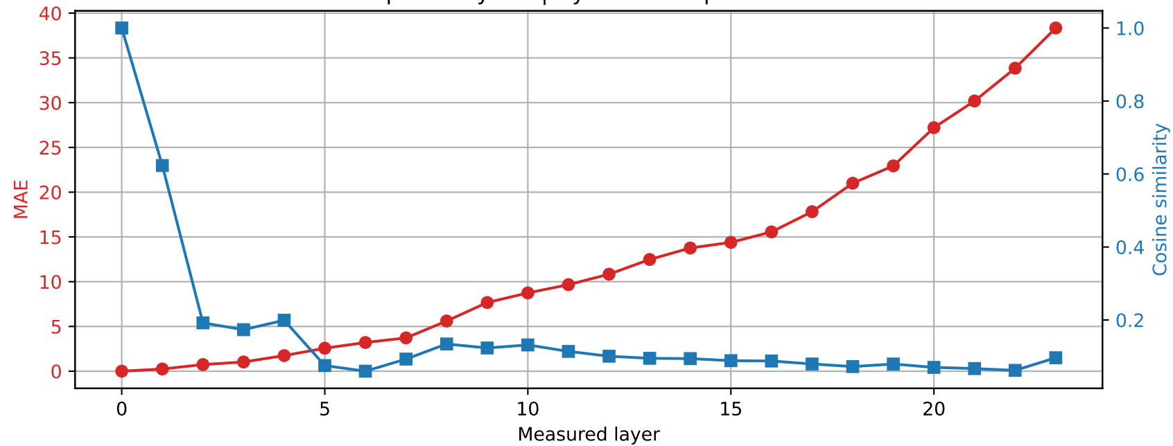
SmolLM2-1.7B-Instruct | Prompt 1 Spared layer 8 | Hybrid vs unquantized
