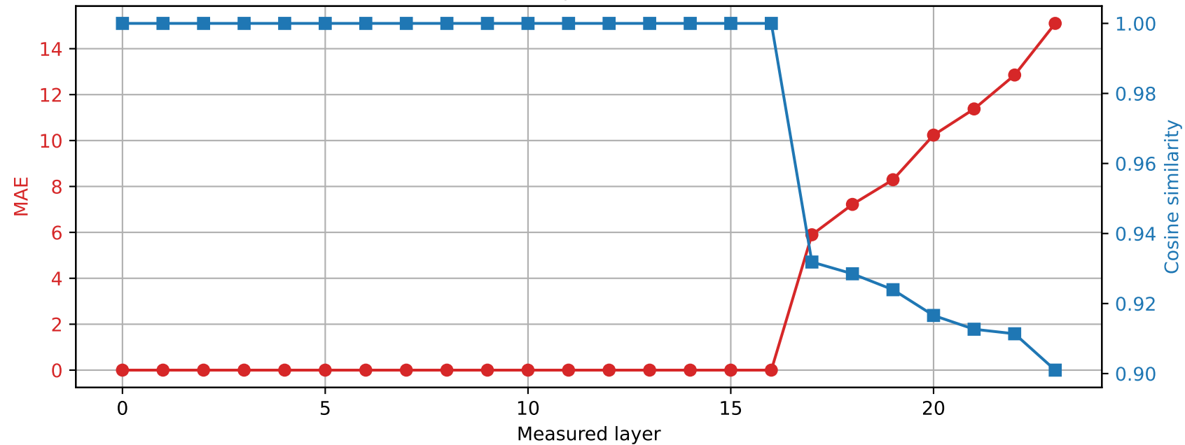
SmolLM2-1.7B-Instruct | Prompt 1 Spared layer 16 | Hybrid vs quantized
