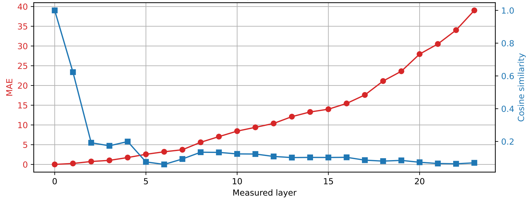
SmolLM2-1.7B-Instruct | Prompt 1 Spared layer 22 | Hybrid vs unquantized
