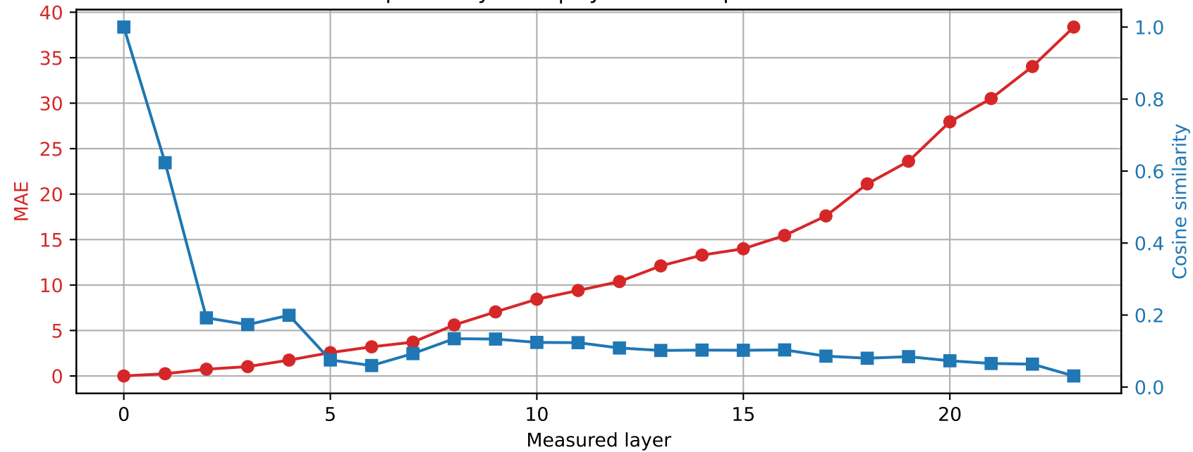
SmolLM2-1.7B-Instruct | Prompt 1 Spared layer 23 | Hybrid vs unquantized
