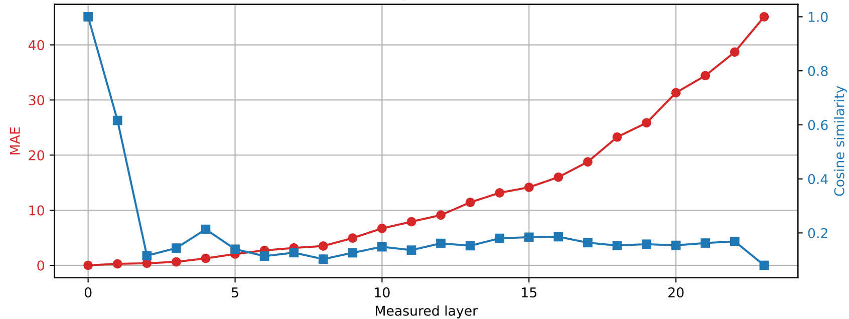
SmolLM2-1.7B-Instruct | Prompt 2 Spared layer 0 | Hybrid vs quantized
