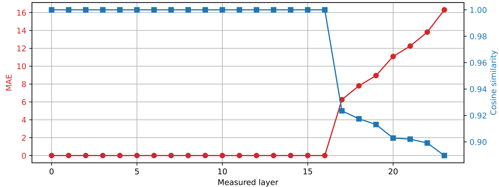
SmolLM2-1.7B-Instruct | Prompt 2 Spared layer 16 | Hybrid vs quantized
