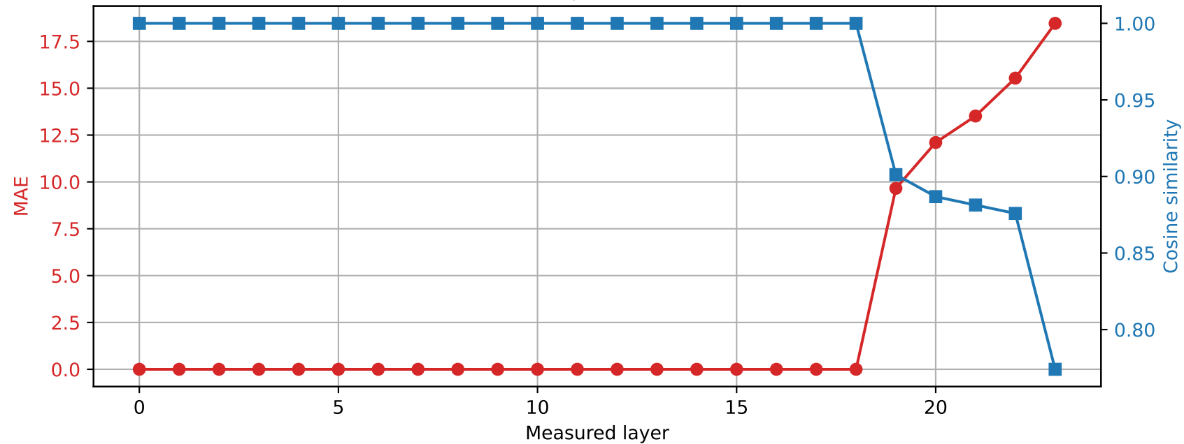
SmolLM2-1.7B-Instruct | Prompt 2 Spared layer 18 | Hybrid vs quantized
