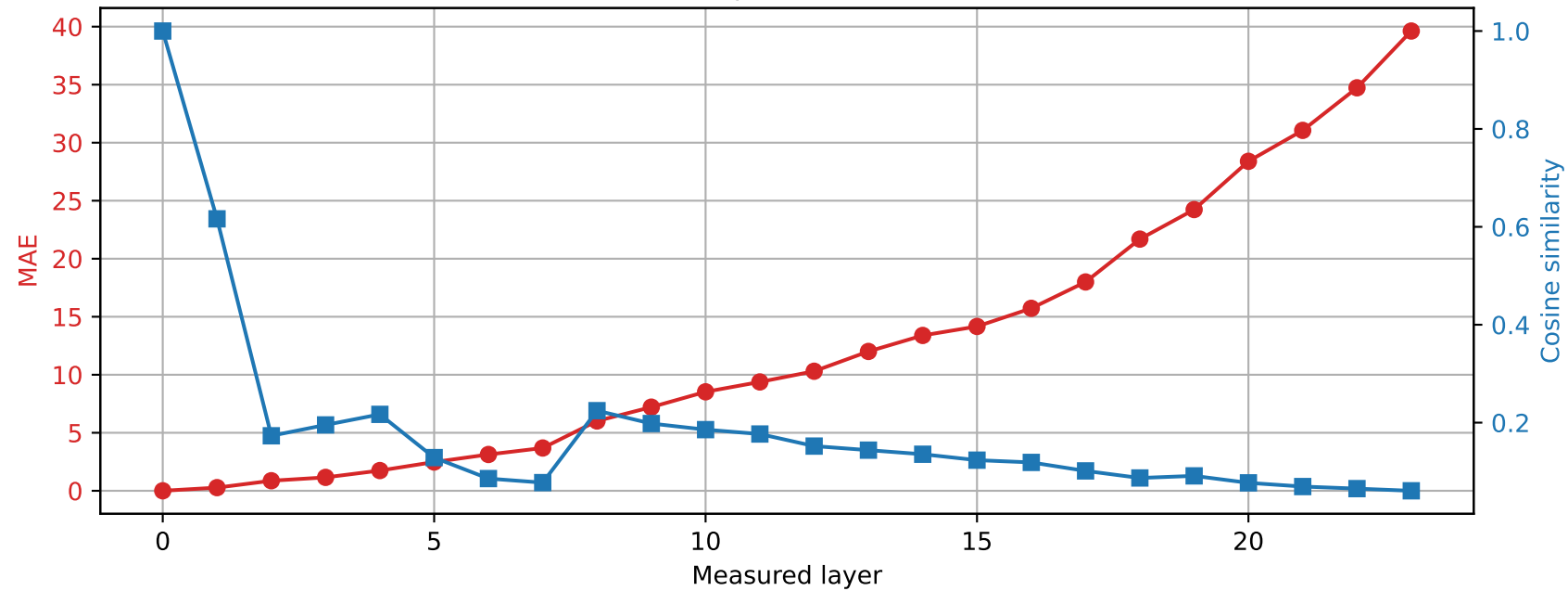
SmolLM2-1.7B-Instruct | Prompt 2 Spared layer 22 | Hybrid vs unquantized
