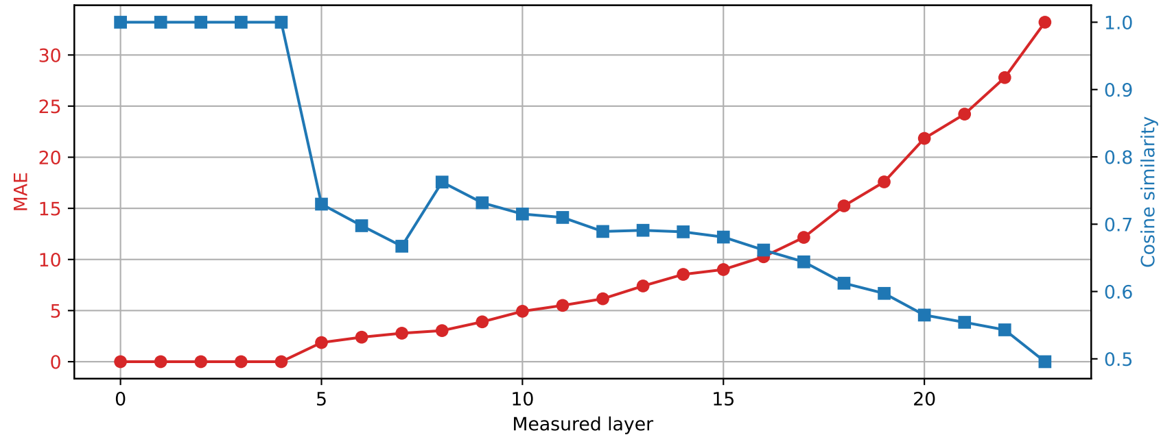
SmolLM2-1.7B-Instruct | Prompt 3 Spared layer 4 | Hybrid vs quantized
