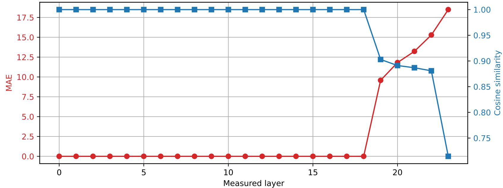
SmolLM2-1.7B-Instruct | Prompt 3 Spared layer 18 | Hybrid vs quantized
