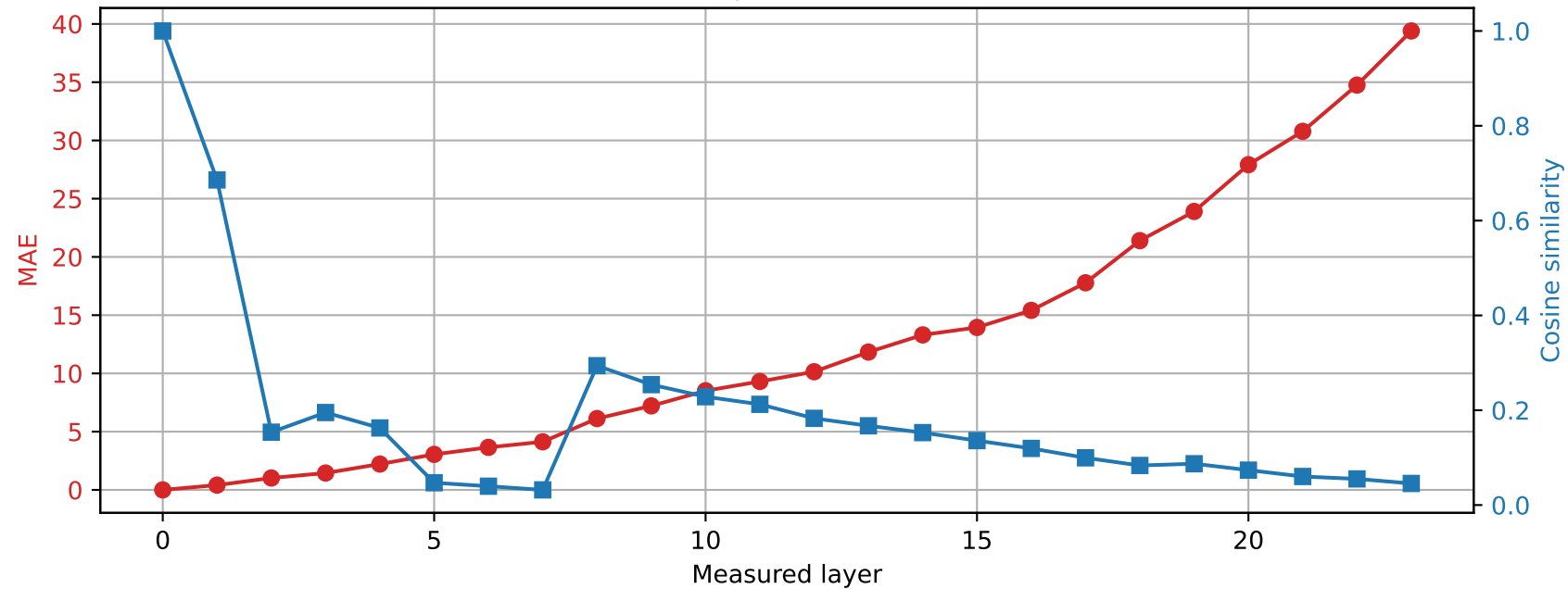
SmolLM2-1.7B-Instruct | Prompt 3 Spared layer 20 | Hybrid vs unquantized
