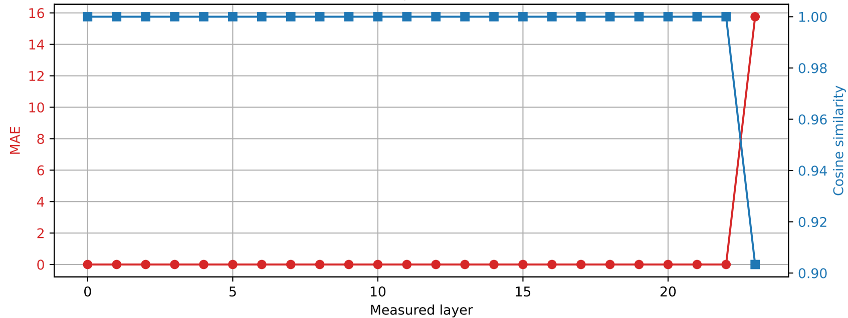
SmolLM2-1.7B-Instruct | Prompt 3 Spared layer 22 | Hybrid vs quantized
