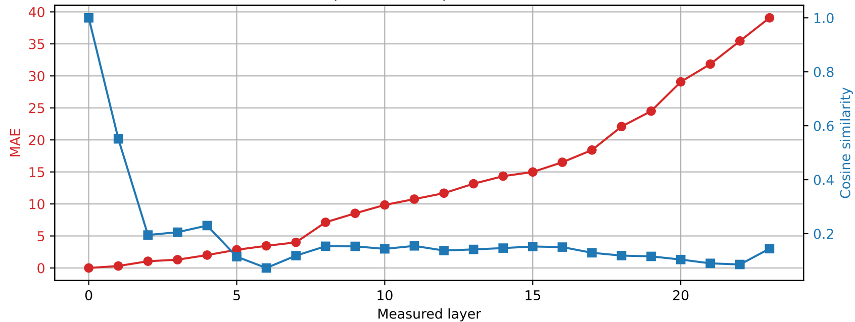
SmolLM2-1.7B-Instruct | Prompt 4 Unquantized vs quantized int4
