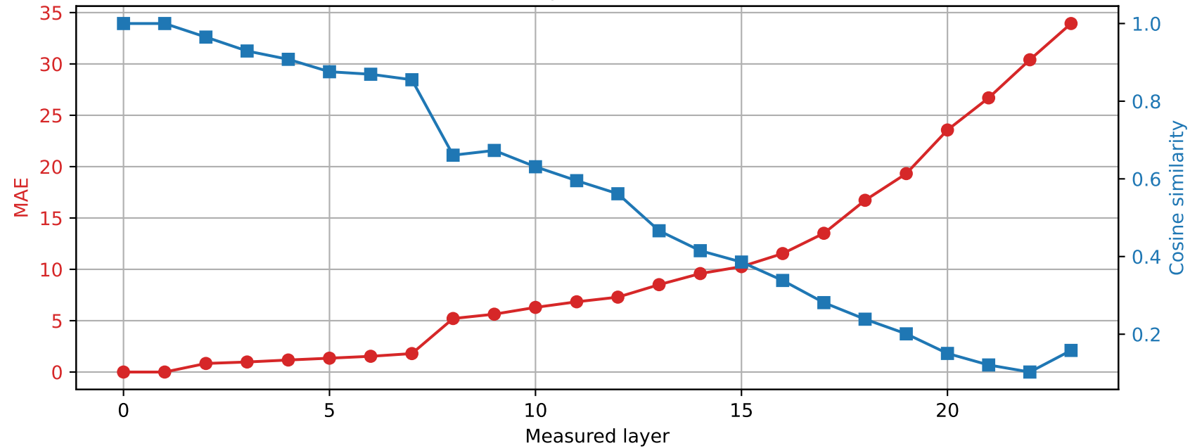
SmolLM2-1.7B-Instruct | Prompt 4 Spared layer 0 | Hybrid vs unquantized
