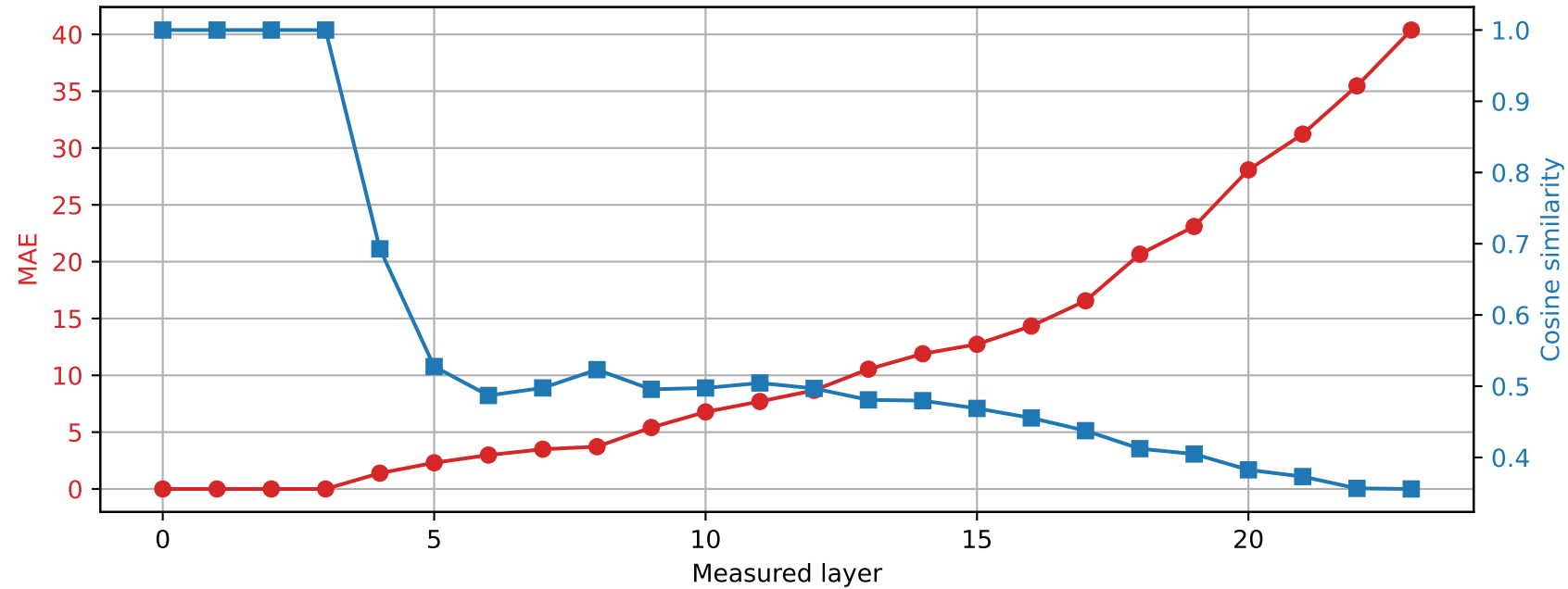
SmolLM2-1.7B-Instruct | Prompt 4 Spared layer 3 | Hybrid vs quantized
