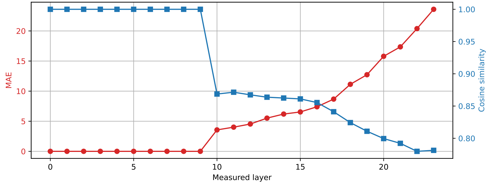
SmolLM2-1.7B-Instruct | Prompt 4 Spared layer 9 | Hybrid vs quantized
