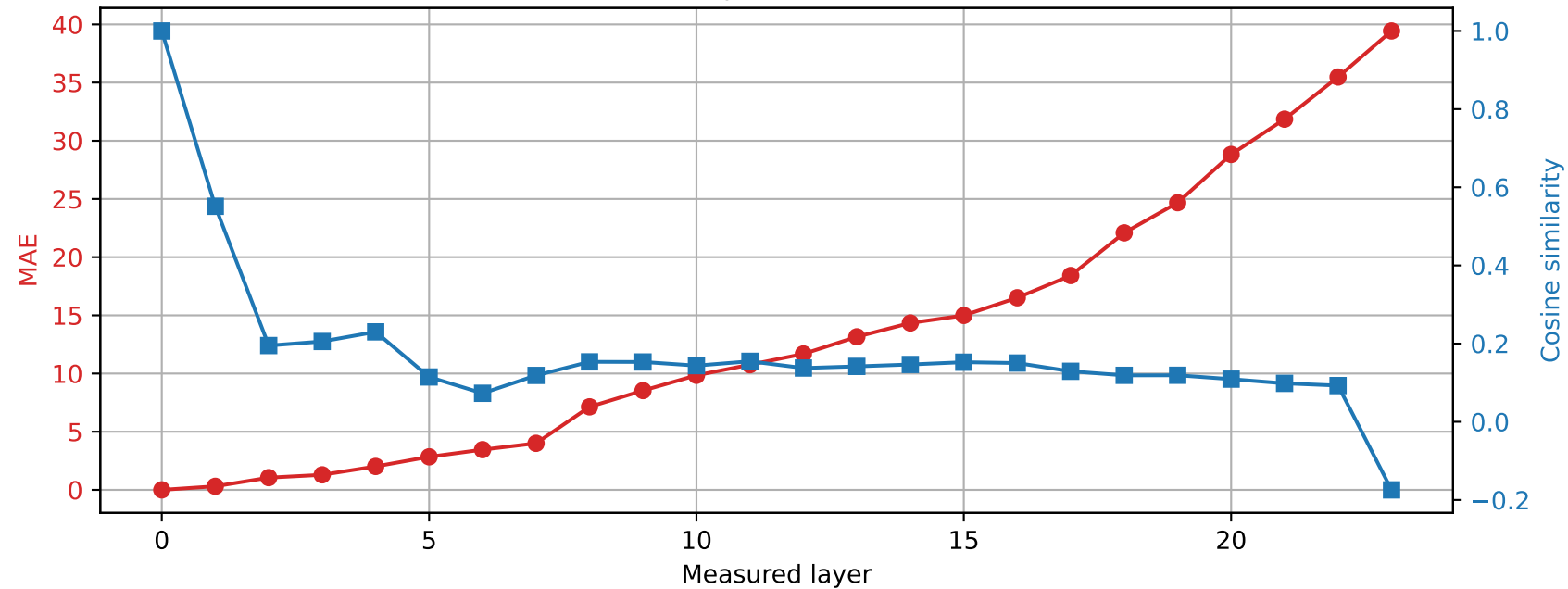
SmolLM2-1.7B-Instruct | Prompt 4 Spared layer 18 | Hybrid vs unquantized
