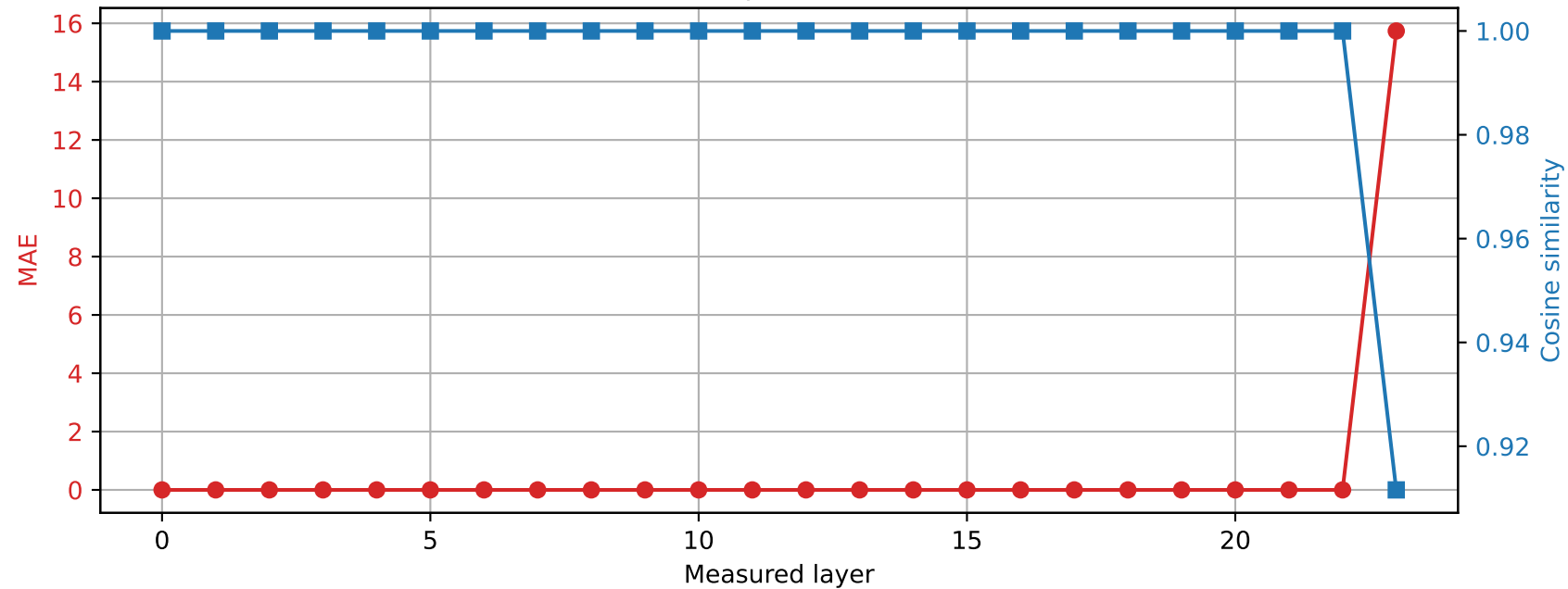
SmolLM2-1.7B-Instruct | Prompt 4 Spared layer 22 | Hybrid vs quantized
