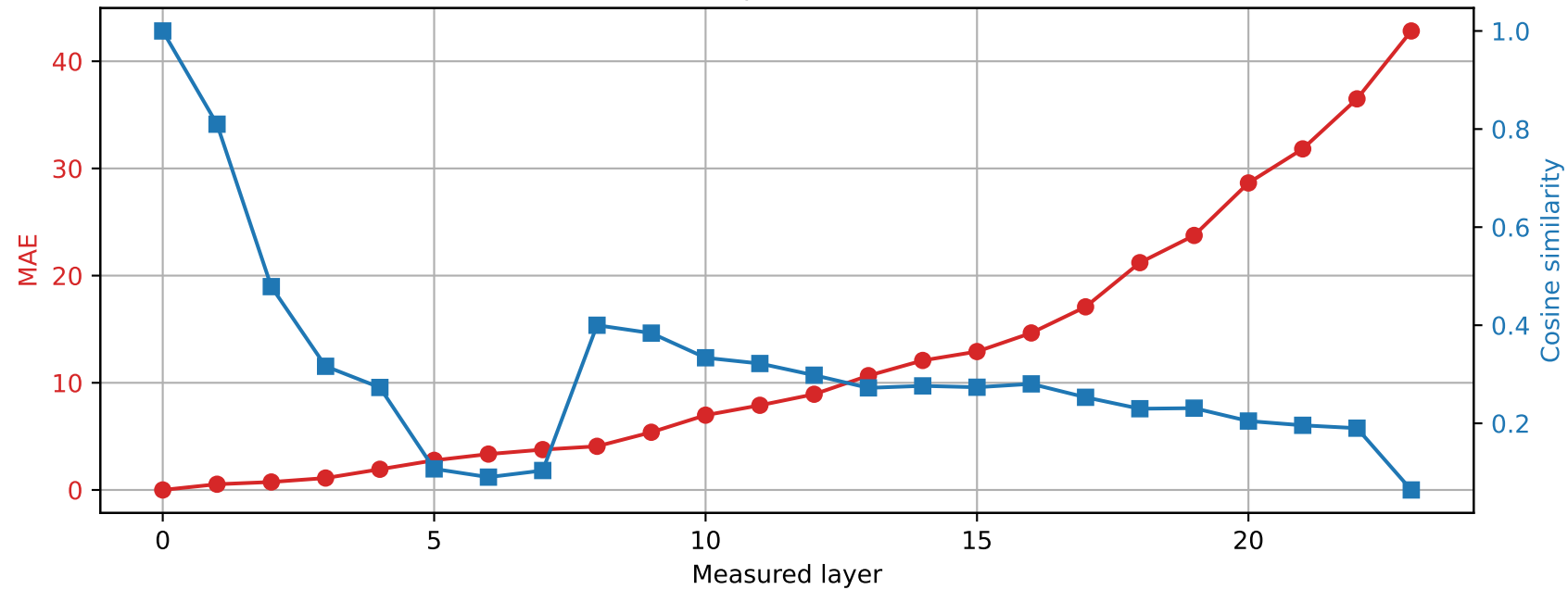
SmolLM2-1.7B-Instruct | Prompt 0 Spared layer 0 | Hybrid vs quantized
