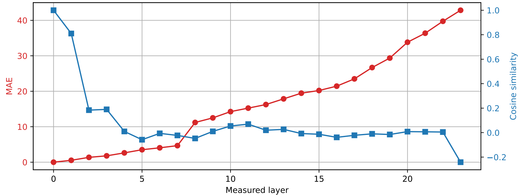
SmolLM2-1.7B-Instruct | Prompt 0 Spared layer 1 | Hybrid vs unquantized
