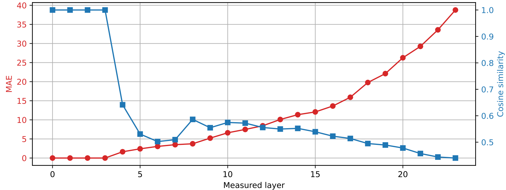
SmolLM2-1.7B-Instruct | Prompt 0 Spared layer 3 | Hybrid vs quantized
