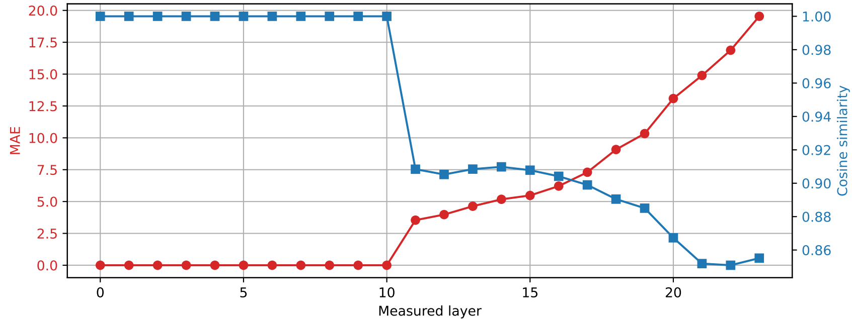
SmolLM2-1.7B-Instruct | Prompt 0 Spared layer 10 | Hybrid vs quantized
