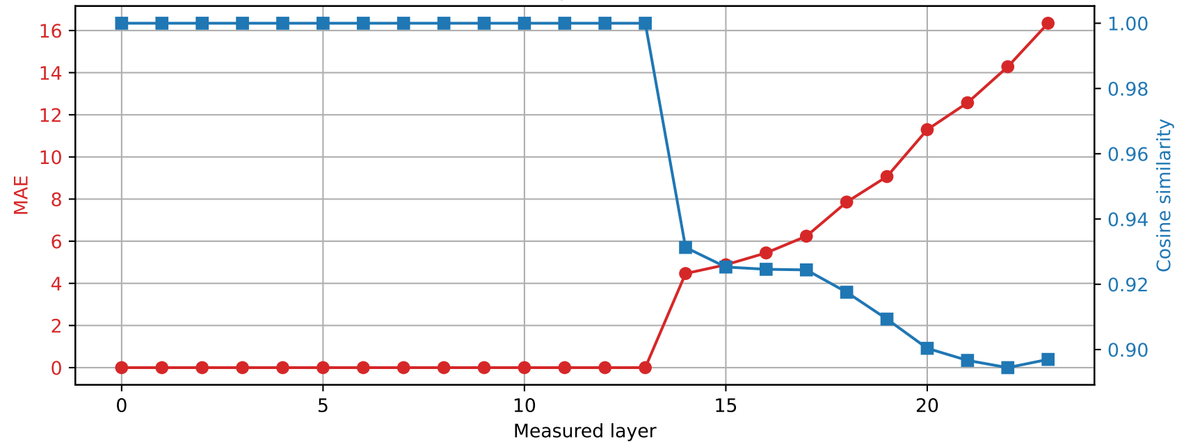
SmolLM2-1.7B-Instruct | Prompt 0 Spared layer 13 | Hybrid vs quantized
