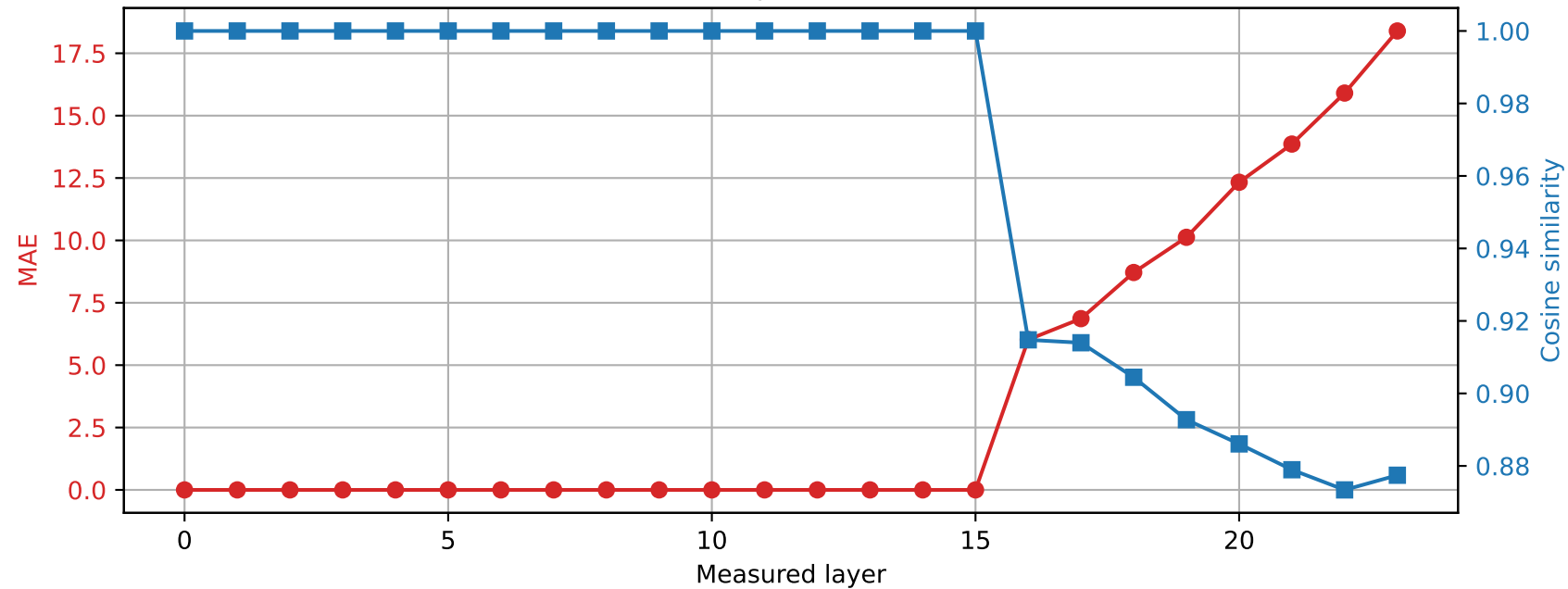
SmolLM2-1.7B-Instruct | Prompt 0 Spared layer 15 | Hybrid vs quantized
