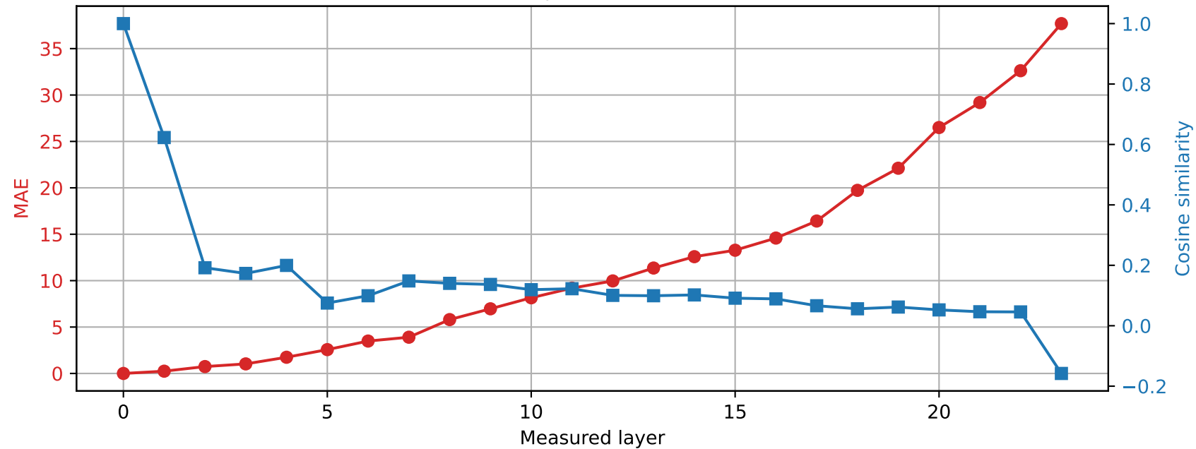
SmolLM2-1.7B-Instruct | Prompt 1 Spared layer 5 | Hybrid vs unquantized
