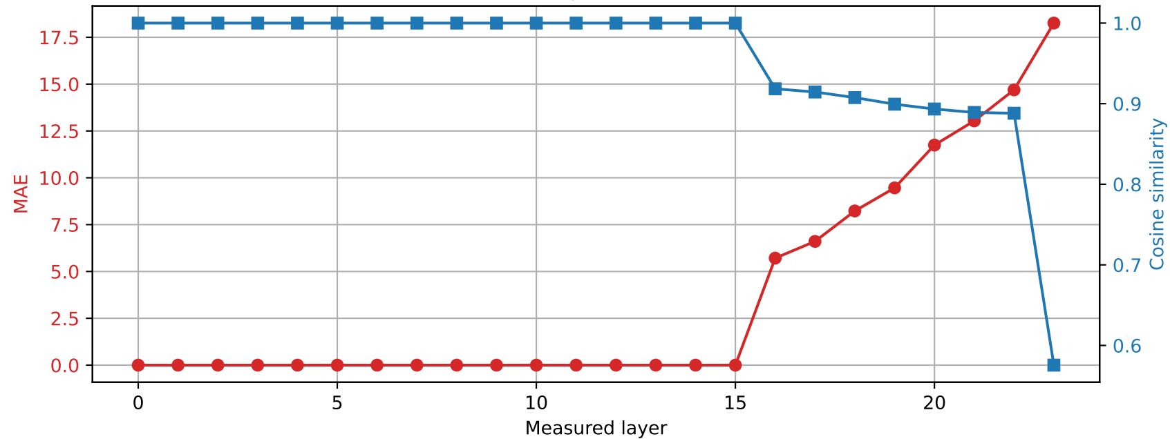
SmolLM2-1.7B-Instruct | Prompt 1 Spared layer 15 | Hybrid vs quantized
