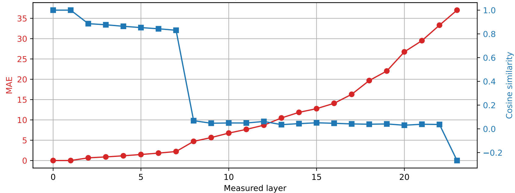
SmolLM2-1.7B-Instruct | Prompt 2 Spared layer 0 | Hybrid vs unquantized
