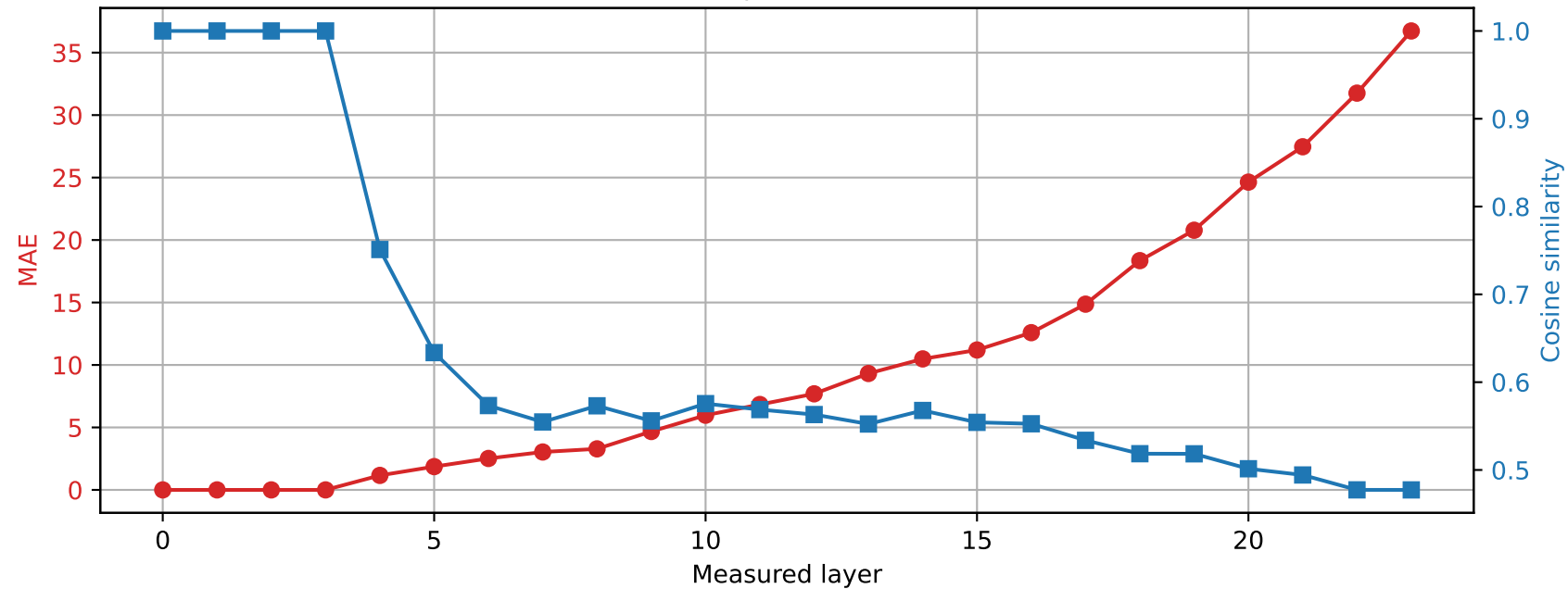
SmolLM2-1.7B-Instruct | Prompt 2 Spared layer 3 | Hybrid vs quantized
