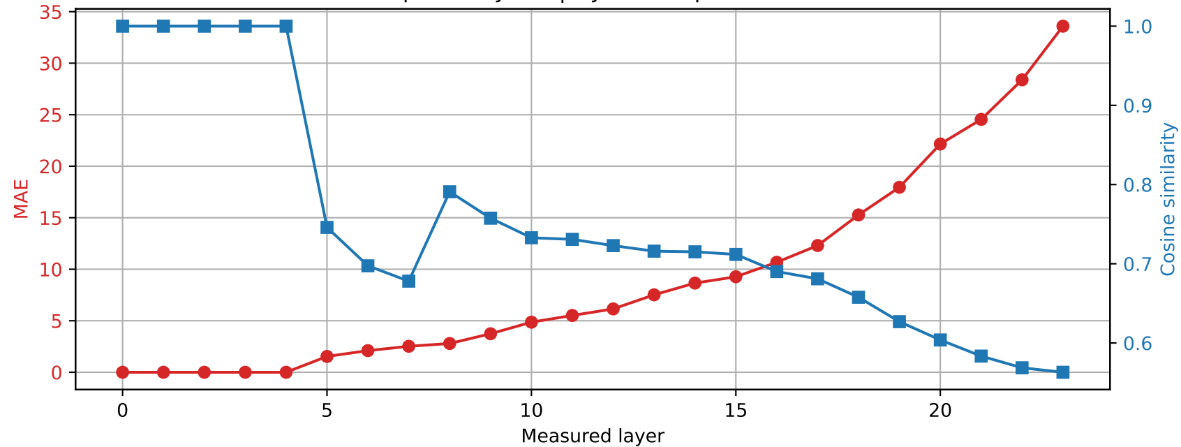
SmolLM2-1.7B-Instruct | Prompt 2 Spared layer 4 | Hybrid vs quantized
