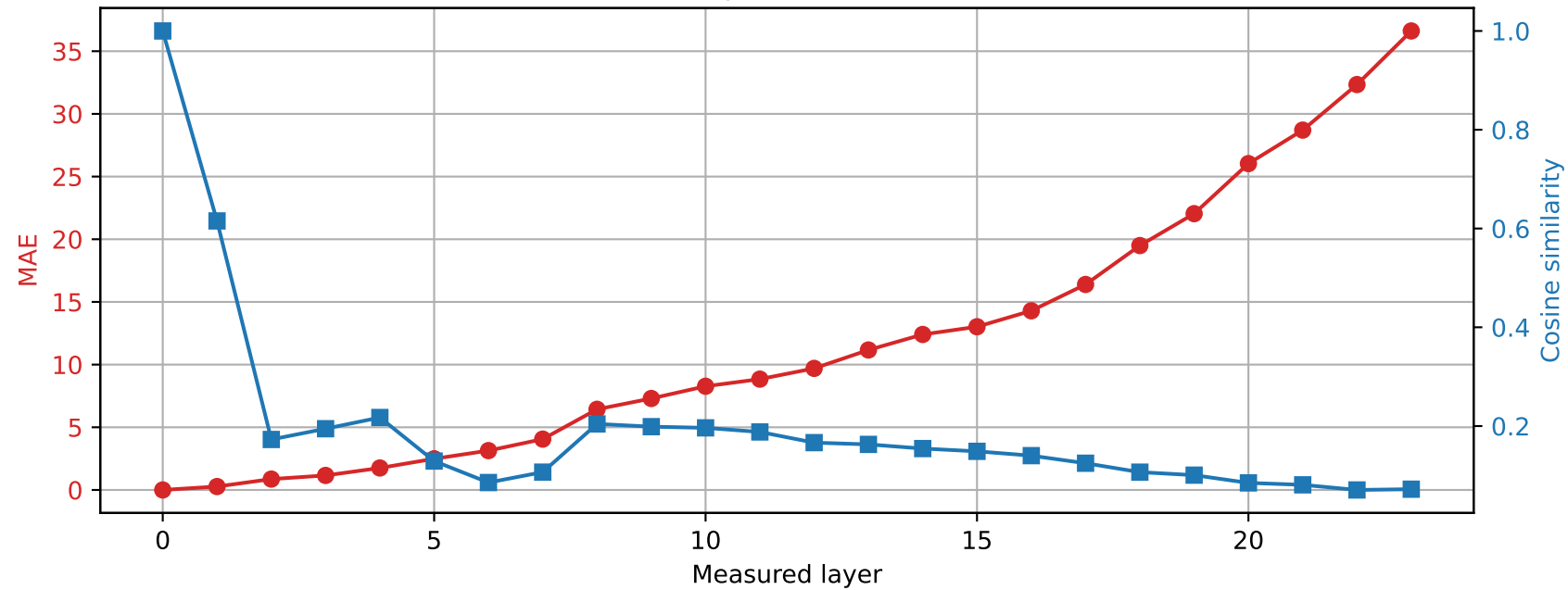
SmolLM2-1.7B-Instruct | Prompt 2 Spared layer 6 | Hybrid vs unquantized
