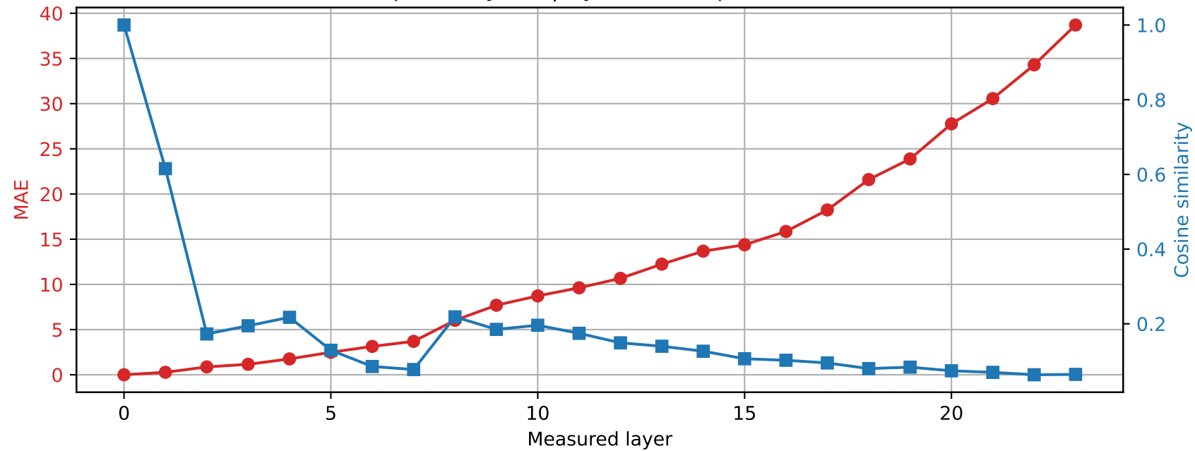
SmolLM2-1.7B-Instruct | Prompt 2 Spared layer 8 | Hybrid vs unquantized
