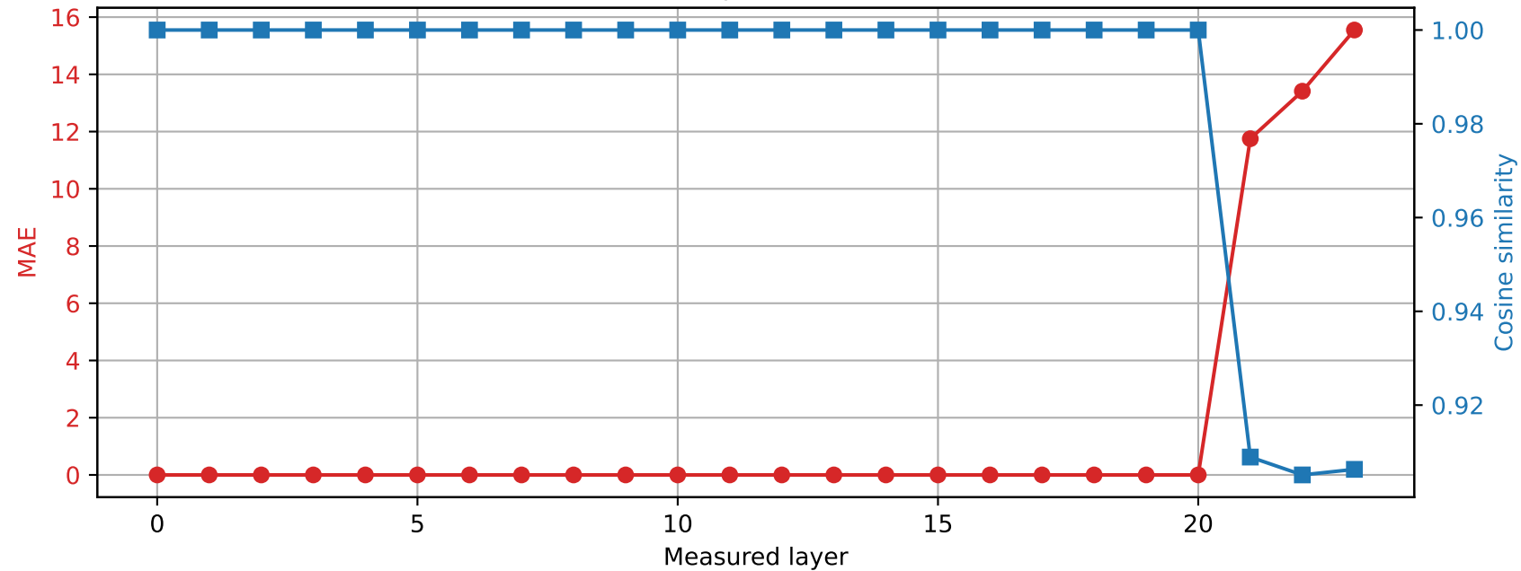
SmolLM2-1.7B-Instruct | Prompt 2 Spared layer 20 | Hybrid vs quantized
