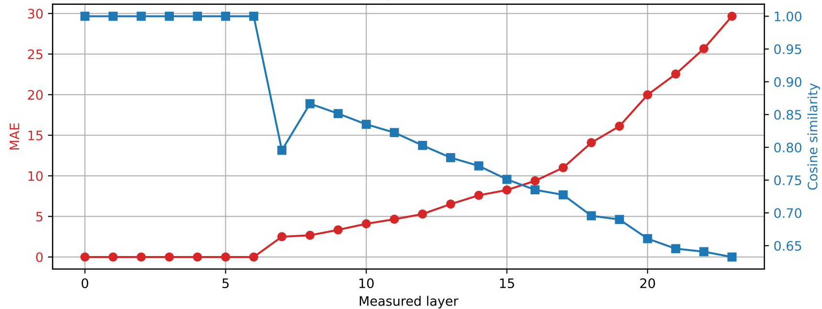
SmolLM2-1.7B-Instruct | Prompt 3 Spared layer 6 | Hybrid vs quantized
