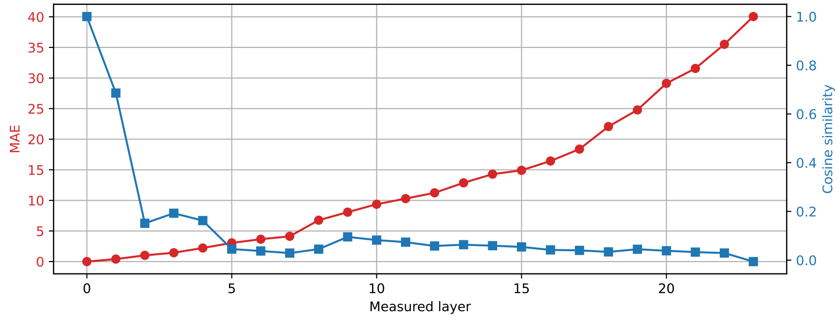
SmolLM2-1.7B-Instruct | Prompt 3 Spared layer 7 | Hybrid vs unquantized
