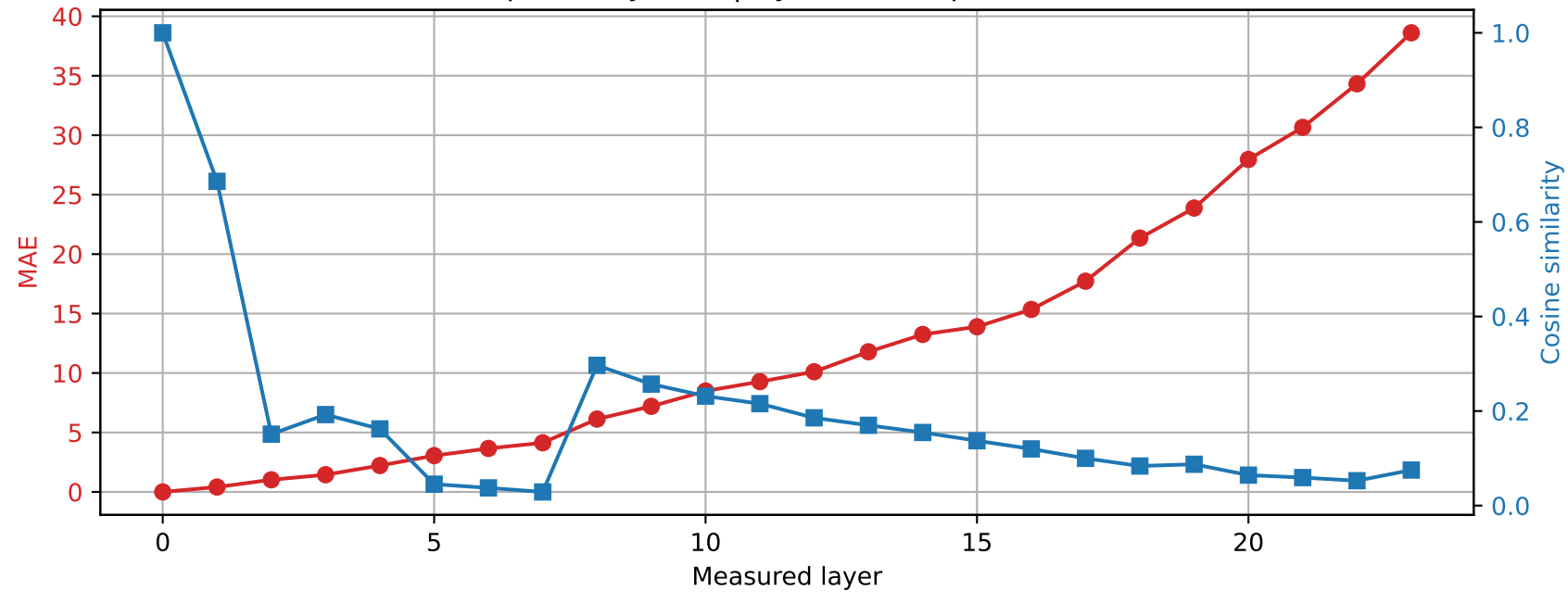
SmolLM2-1.7B-Instruct | Prompt 3 Spared layer 19 | Hybrid vs unquantized
