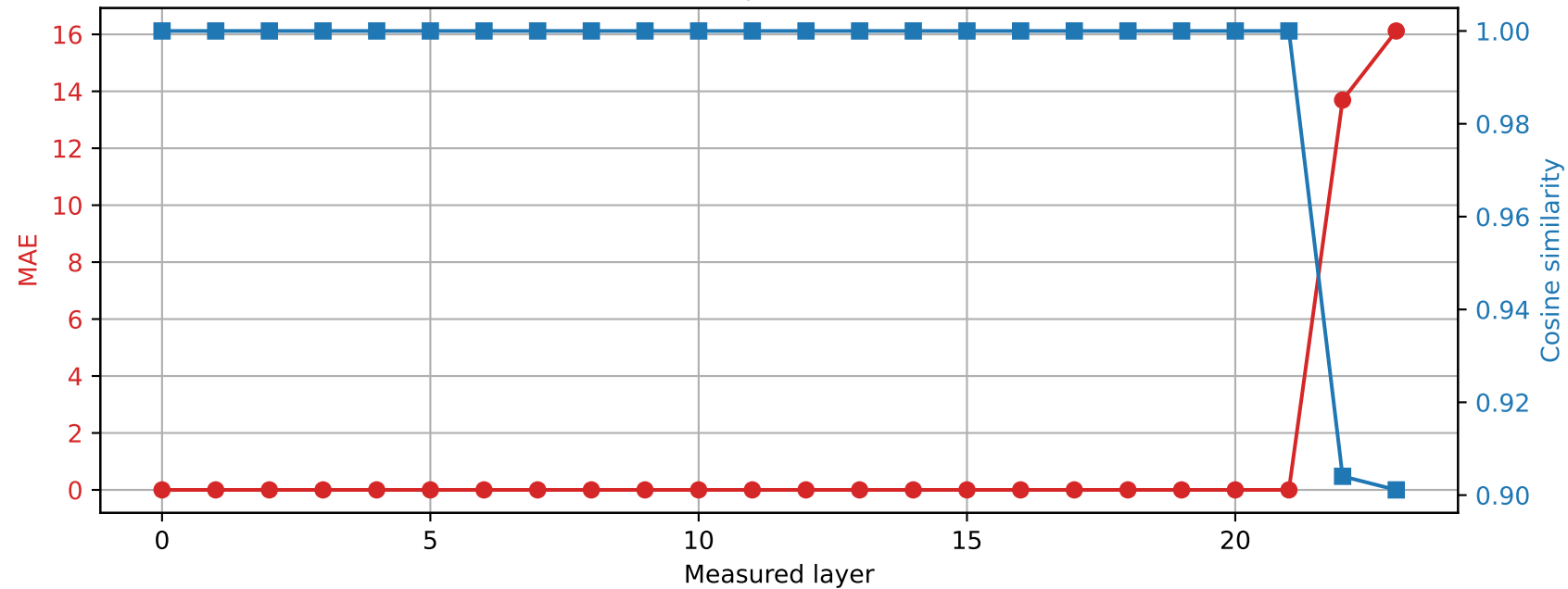
SmolLM2-1.7B-Instruct | Prompt 3 Spared layer 21 | Hybrid vs quantized
